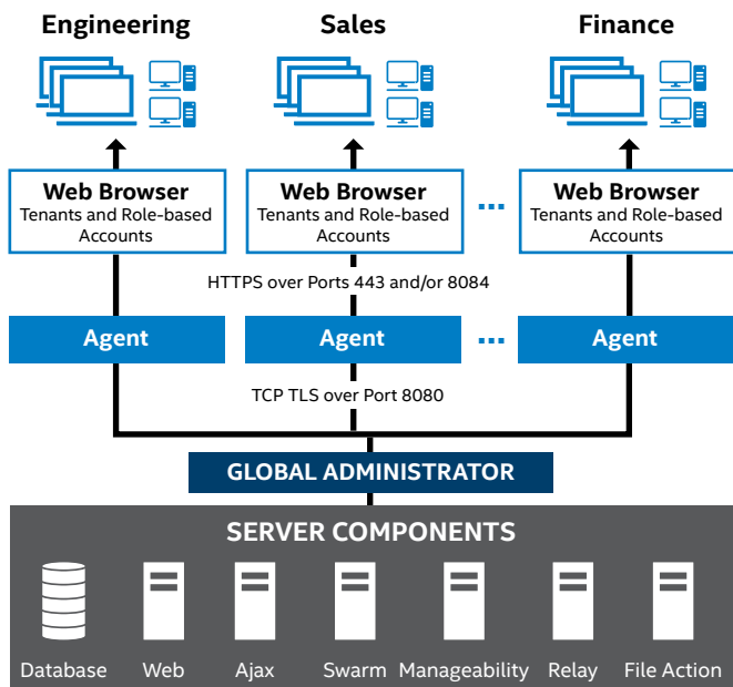
Figure 3. Single-instance base server components allow global administrators to define and manage tenant environments and tenant administrators in any deployment scenario.
